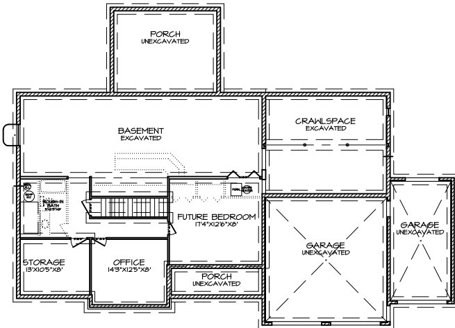
2 FOUNDATION PLAN A-2
